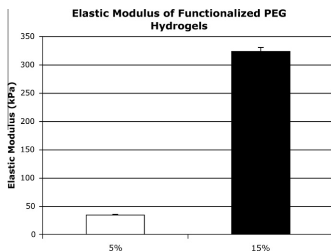
Fig. 3. Stiffness of the two weight–volume fraction functionalized PEG gels as determined by the elastic modulus during uniaxial tensile testing. Four PEG hydrogel samples of each weight–volume fraction were tested.
